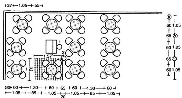
⑤ Minimal table spacing
